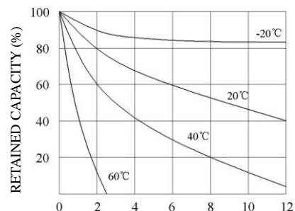
SELF DISCHARGE RATE AT VARIOUS TEMPERATURES
