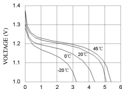
DISCHARGE CURVE AT VARIOUS TEMPERATURES (50mA)
