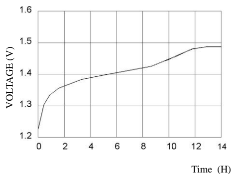
TYPICAL CHARGE CURVE (25mA)
