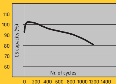
TAB Traction GEL batteries (PzV, PzVB) C5 capacity during life
