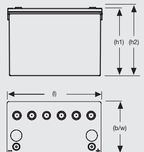
XL12V85
