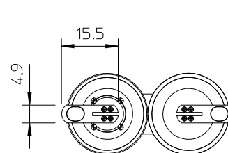
Languette Clip 4.9x0.6 x15.5 Faston tag 4.9x0.6x15.5
