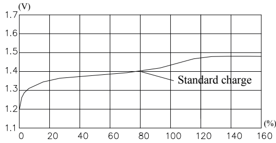
Charge Curve
