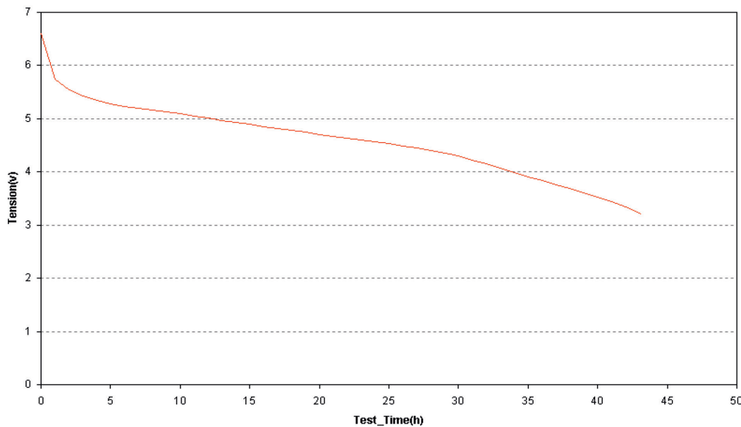
Decharge sur 10ohms
